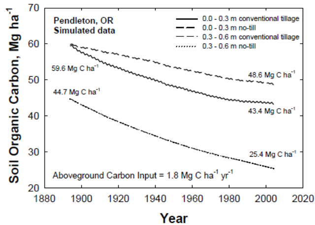
Figure 26.3. Simulated soil carbon evolution at Pendleton, Oregon, under conventional till and no-till management. The initial soil carbon corresponds to that of the original sagebrush-grassland undisturbed soil. The rotation was winter wheat - summer fallow with yields adjusted for current technological conditions. It was assumed that, on average, winter wheat crops leave 8.4 Mg of biomass per harvest year, corresponding to average inputs of aboveground residues of 1.8 Mg C y -1 . The numbers on the graph show initial and final soil carbon in the top 0.3 m and in the 0.3 to 0.6 m layer. The results for the layer 0.3 – 0.6 m for both systems are almost identical and only one line is shown.
