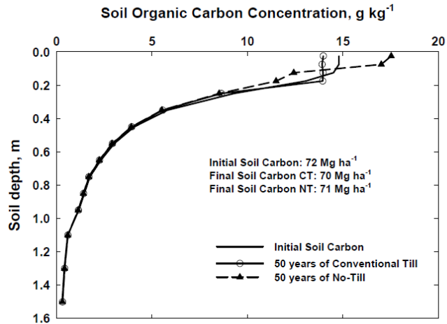
Figure 26.5. Stratification of soil carbon after 50 years of no-till as simulated with the C-Farm model. Both the simulation with conventional tillage (CT) and no-till (NT) started with the same soil profile. Carbon inputs were kept almost identical, although inputs for conventional tillage treatment were slightly greater (< 1%) than under no-till. Including shoots and roots, inputs totalize approximately 4 Mg C ha -1 y -1 .
