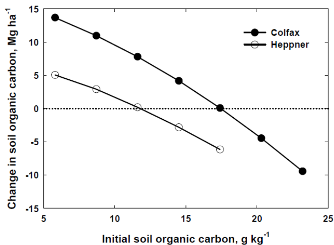
Figure 26.4. Simulated 50-year change of organic carbon ( C_s ) in the top 0.3 m of soil as a function of initial C_s at two locations: Colfax, Washington and Heppner, Oregon. Residue inputs (shoots plus roots) were 3.2 and 1.4 \text{Mg C ha}^{-1} \text{y}^{-1} for Colfax and Heppner, respectively.
